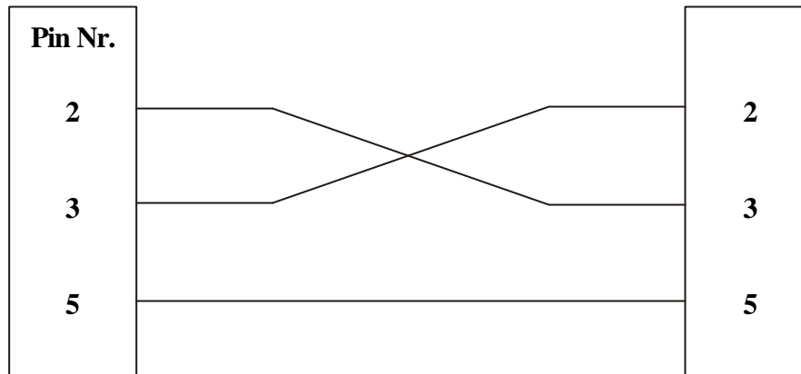
Null- Modem Kabel
